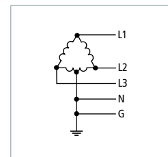
three-phase; 5 wire Delta "Highleg" (3 Ph Δ, 4 W + G) 120 V / 240 V
