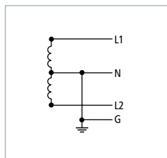
single-phase; 4 wire Split Phase or Edison (1 Ph, 3 W + G) 120 V / 240 V
