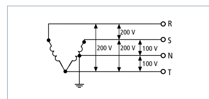
three-phase + single-phase 100 V / 200 V; 200 V
