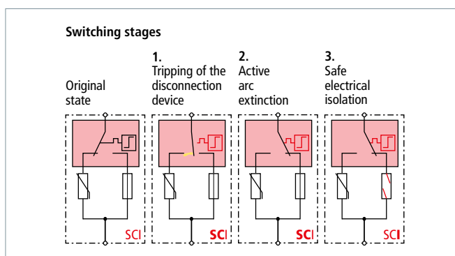
Three-step d.c. switching device (patented SCI principle)
