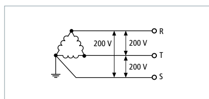
three-phase; 3 wire (3 Ph, 3 W) 200 V
