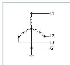
three-phase; 4 wire (3 Ph Y, 3 W + G) 480 V
