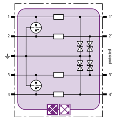
Pluggable SPDs – DIN Rail Mounted
