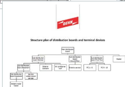
Structure plan
