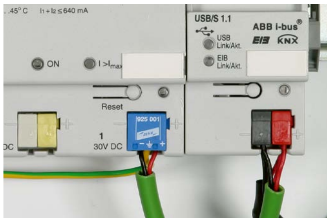
Protection of a KNX power supply unit by means of a BUSector surge arrester mounted in the standard bus terminal slot.
