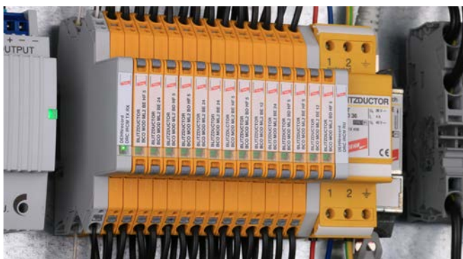
BLITZDUCTORconnect for protecting measuring and control systems
