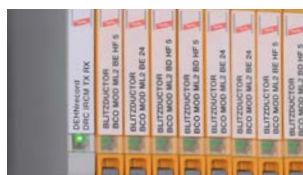
Connect = Protect Simple status message with monitoring unit for arrester groups
