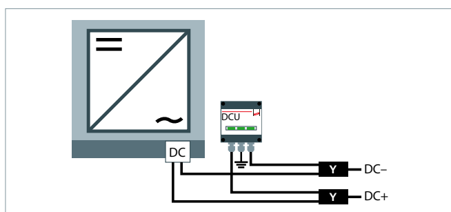
Application: One string per d.c. input (MPP tracker) of the inverter.
