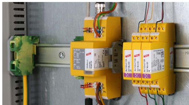
Space-saving and application-optimised 3-in-1 DEHNvario arrester for analogue camera systems.
