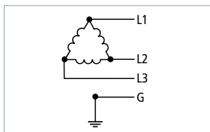
three-phase; 4 wire Delta "Ungrounded" (3 Ph Δ, 3 W + G) 240 V 480 V
