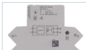
Simple maintenance Remote signalling of the status of arrester groups (break contact)
