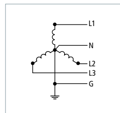
three-phase; 5 wire (3 Ph Y, 4 W + G) 120 V / 208 V 277 V / 480 V
