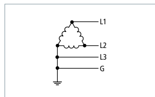
three-phase; 4 wire Delta "Grounded Corner" (3 Ph Δ, 3 W + G) 240 V 480 V
