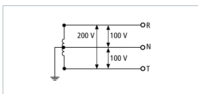
single-phase; 3 wire (1 Ph, 3 W) 100 V / 200 V
